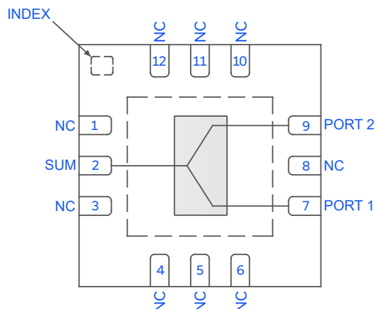
Figure 1. GP2Y1A+ Functional Diagram
