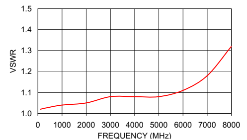
GAT-7+ VSWR
