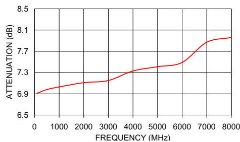
GAT-7+ ATTENUATION
