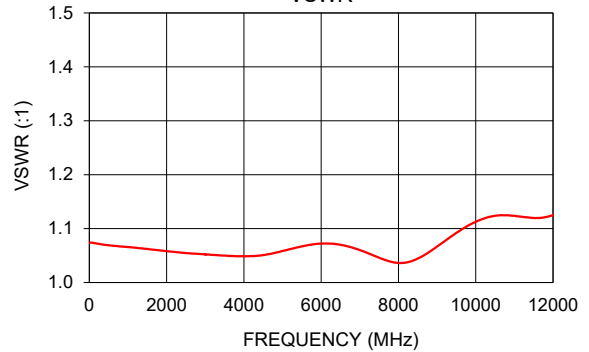
FW-5A+ VSWR
