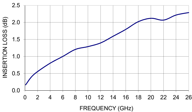
FLC-3FT-SMSM+ INSERTION LOSS
