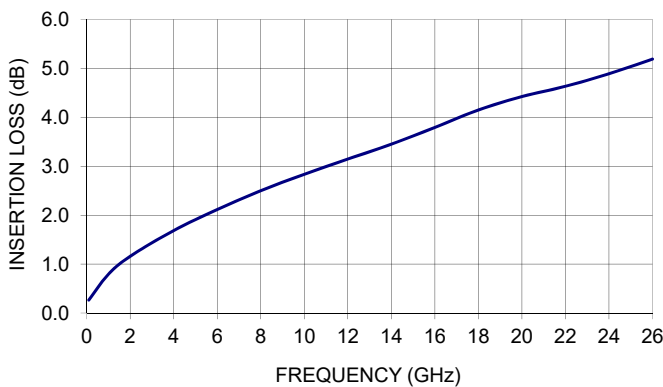
FLC-2M-SMSM+ INSERTION LOSS
