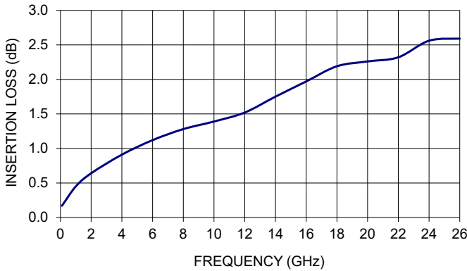
FLC-1M-SMSM+ INSERTION LOSS
