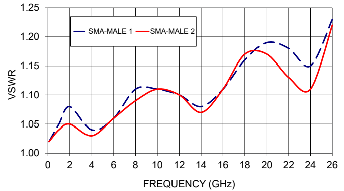
FLC-1M-SMSM+ VSWR
