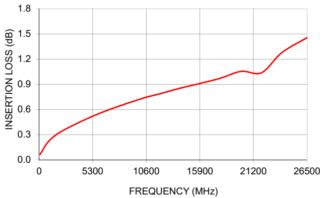
FL86-12SMP+ INSERTION LOSS
