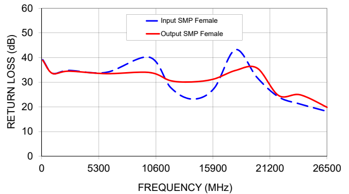
FL86-12SMP+ RETURN LOSS
