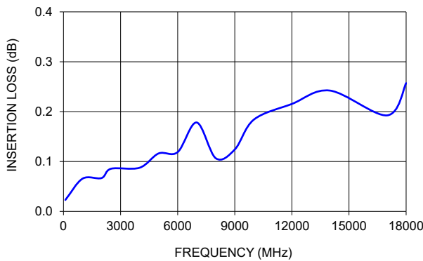
FL141-6SMNM+ INSERTION LOSS
