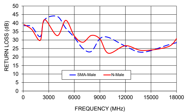
FL141-6SMNM+ RETURN LOSS
