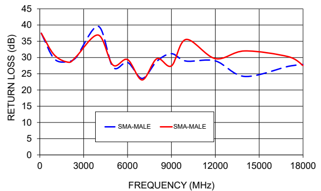
FL141-6SM+ RETURN LOSS
