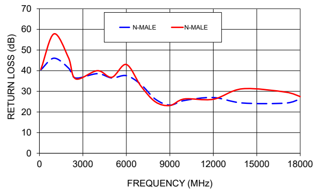
FL141-6NM+ RETURN LOSS
