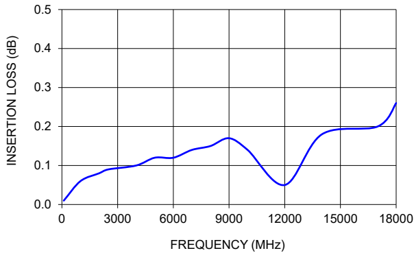
FL141-6NM+ INSERTION LOSS
