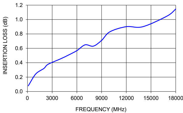
FL141-24SMNM+ INSERTION LOSS
