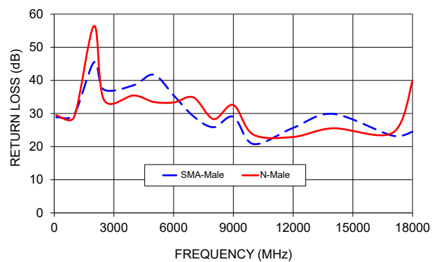
FL141-24SMNM+ RETURN LOSS
