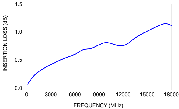
FL141-24NM+ INSERTION LOSS
