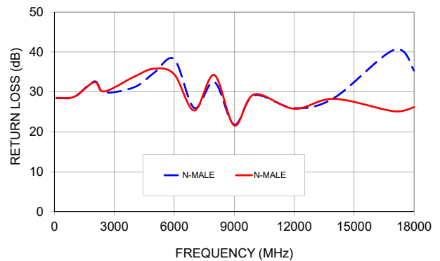
FL141-24NM+ RETURN LOSS
