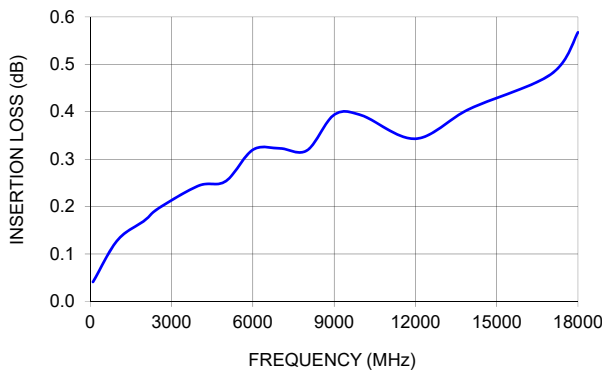
FL141-12NM+ INSERTION LOSS
