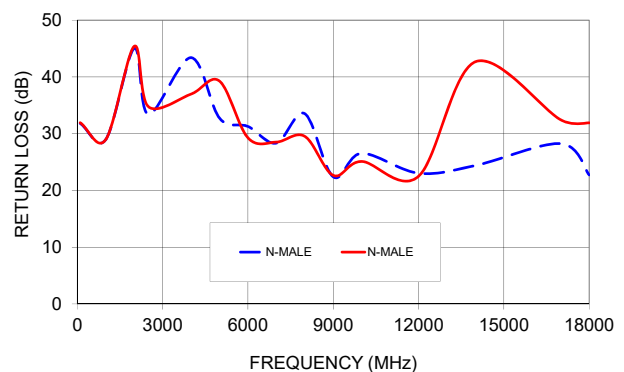
FL141-12NM+ RETURN LOSS
