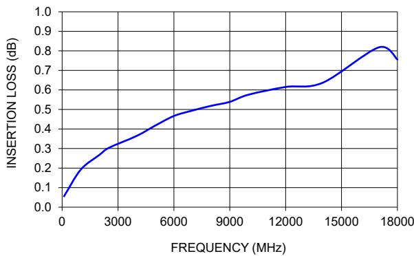
FL086-12NM+ INSERTION LOSS
