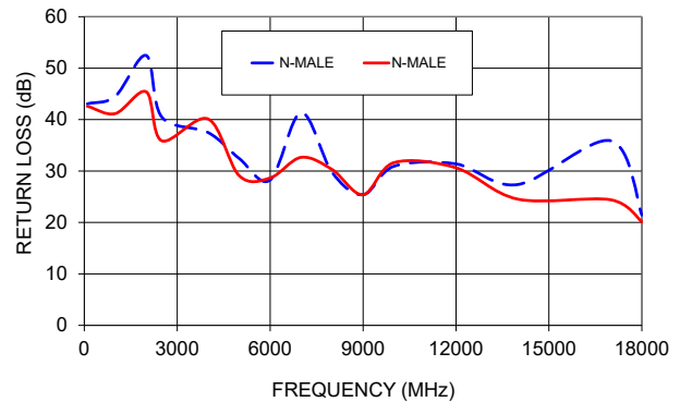
FL086-12NM+ RETURN LOSS
