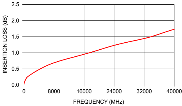
FL086-12KM+ INSERTION LOSS
