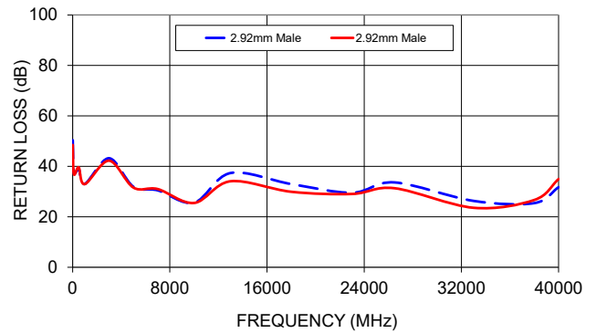
FL086-12KM+ RETURN LOSS
