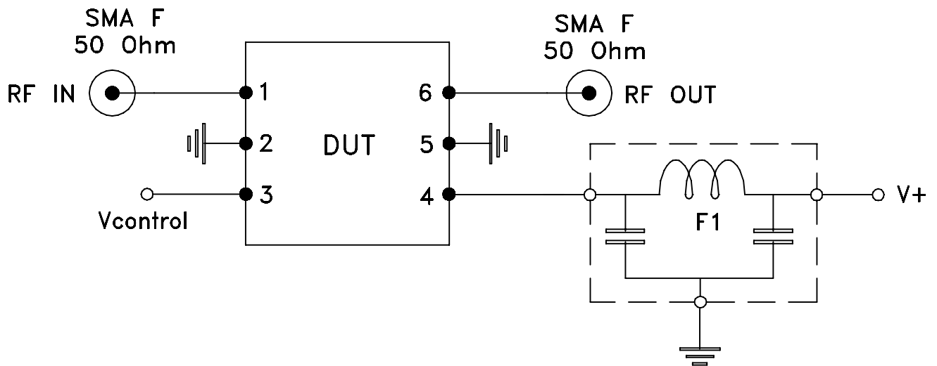
Schematic Diagram
