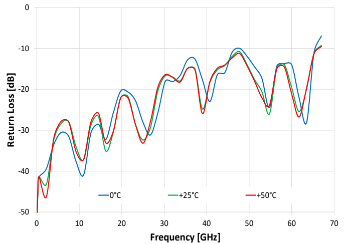
Return Loss @ RF2 over Temperature (RF2 Terminated)
