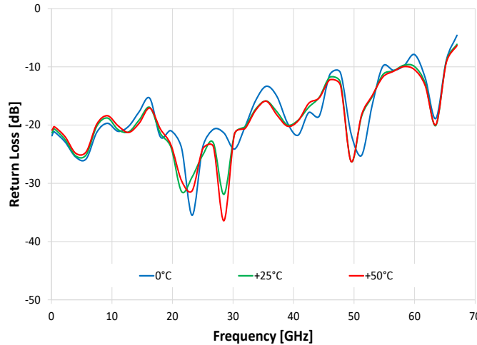
Return Loss @ RF1 over Temperature (RF1 Active)
