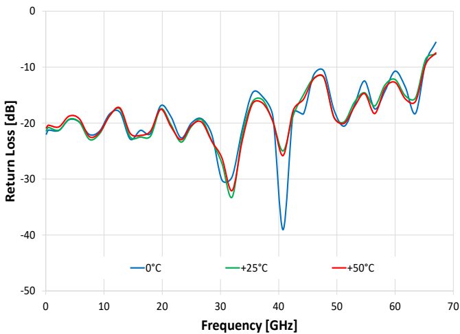
Return Loss @ RF2 over Temperature (RF2 Active)
