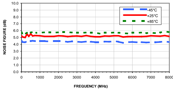
NOISE FIGURE vs. FREQUENCY & TEMPERATURE CURRENT = 50 mA
