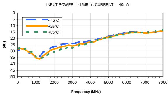
INPUT RETURN LOSS vs. TEMPERATURE
