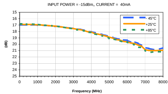
ISOLATION vs. TEMPERATURE
