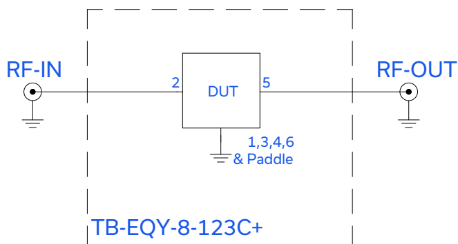
Figure 2. EQY-8-123C+ Evaluation and Application Circuit
