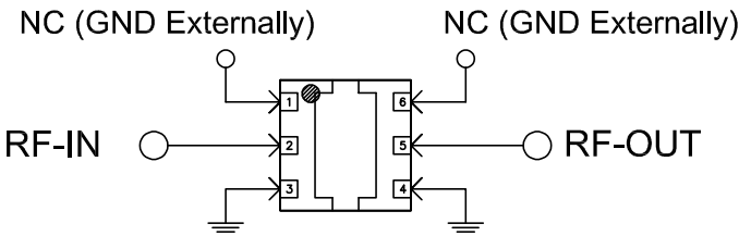
SCHEMATIC DIAGRAM (SCALE 5:1)
