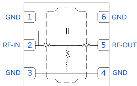
Figure 1. EQY-5-123+ Functional Diagram
