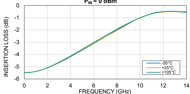
INSERTION LOSS vs. TEMPERATURE
