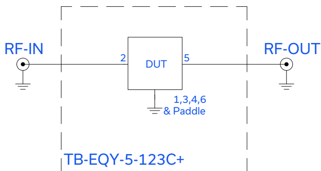
Figure 2. EQY-5-123C+ Evaluation and Application Circuit
