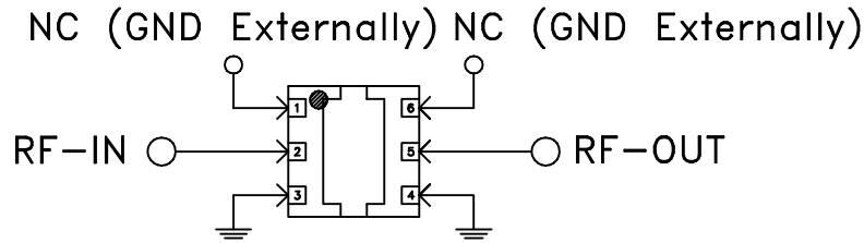
SCHEMATIC DIAGRAM (SCALE 5:1)
