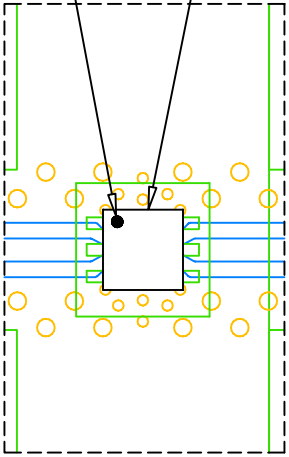
DETAIL "A" (SCALE 5:1)
