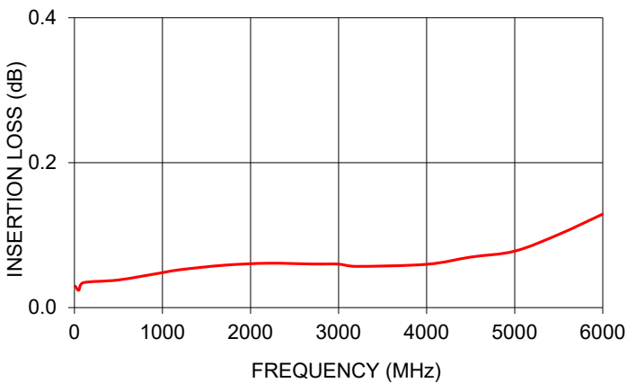
EQY-0-63+ INSERTION LOSS
