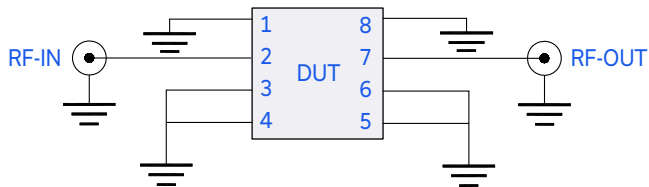
Fig 1. Block Diagram of Test Circuit used for characterization. Test Board TB-EQY-0-63+ Conditions: Attenuation & Return Loss P_{IN}=0 dBm
