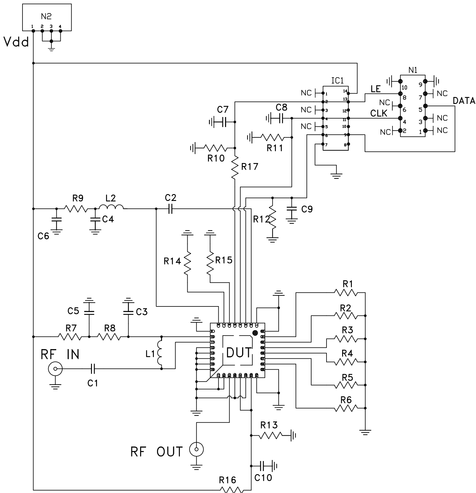
SCHEMATIC DIAGRAM
