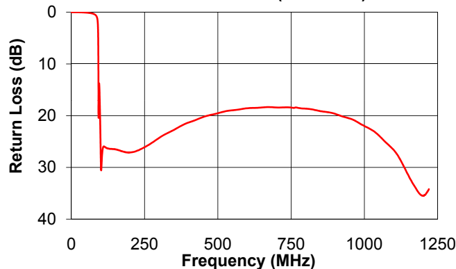
DPB85102-75+ HIGH PASS PORT RETURN LOSS ( P_{in}=0dBm )
