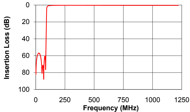
DPB85102-75+ HIGH PASS PORT INSERTION LOSS ( P_{in}=0dBm )
