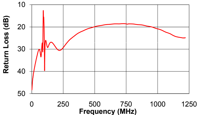
DPB85102-75+ COMMON PORT RETURN LOSS ( P_{in}=0dBm )
