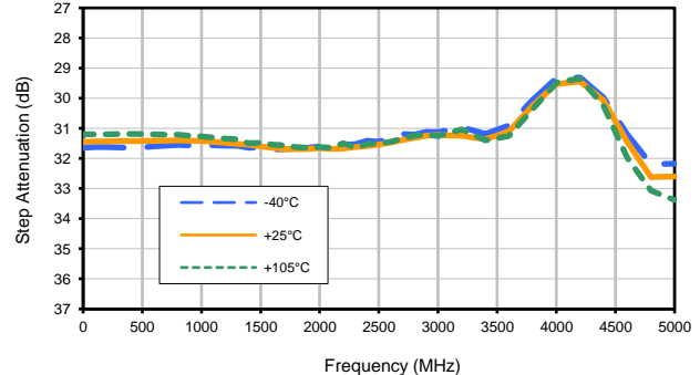
Step Attenuation (31.5dB)
