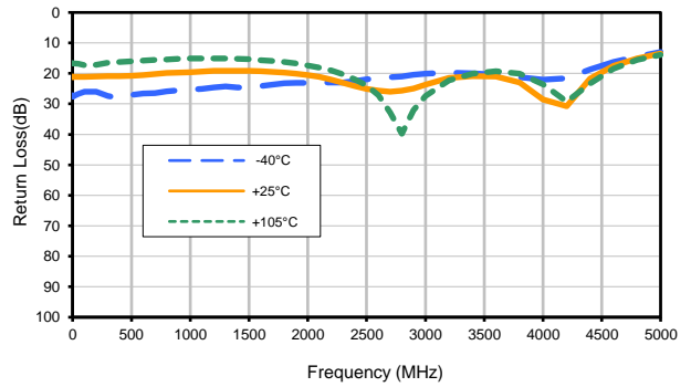
Input Return Loss (31.5dB)
