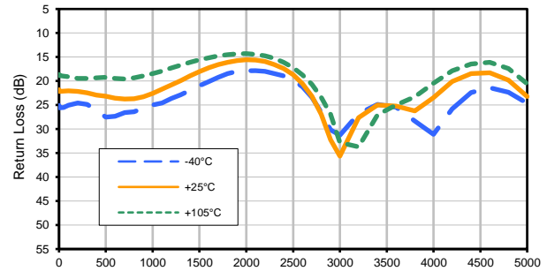
Output Return Loss (2dB)
