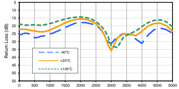
Output Return Loss (2dB)
