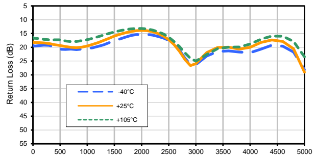
Output Return Loss (0.5dB)
