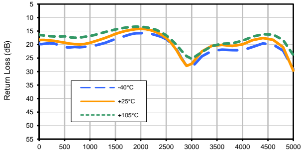
Output Return Loss (1dB)
