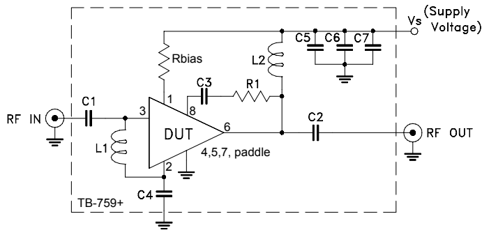
Fig 1. Application and Characterization circuit
