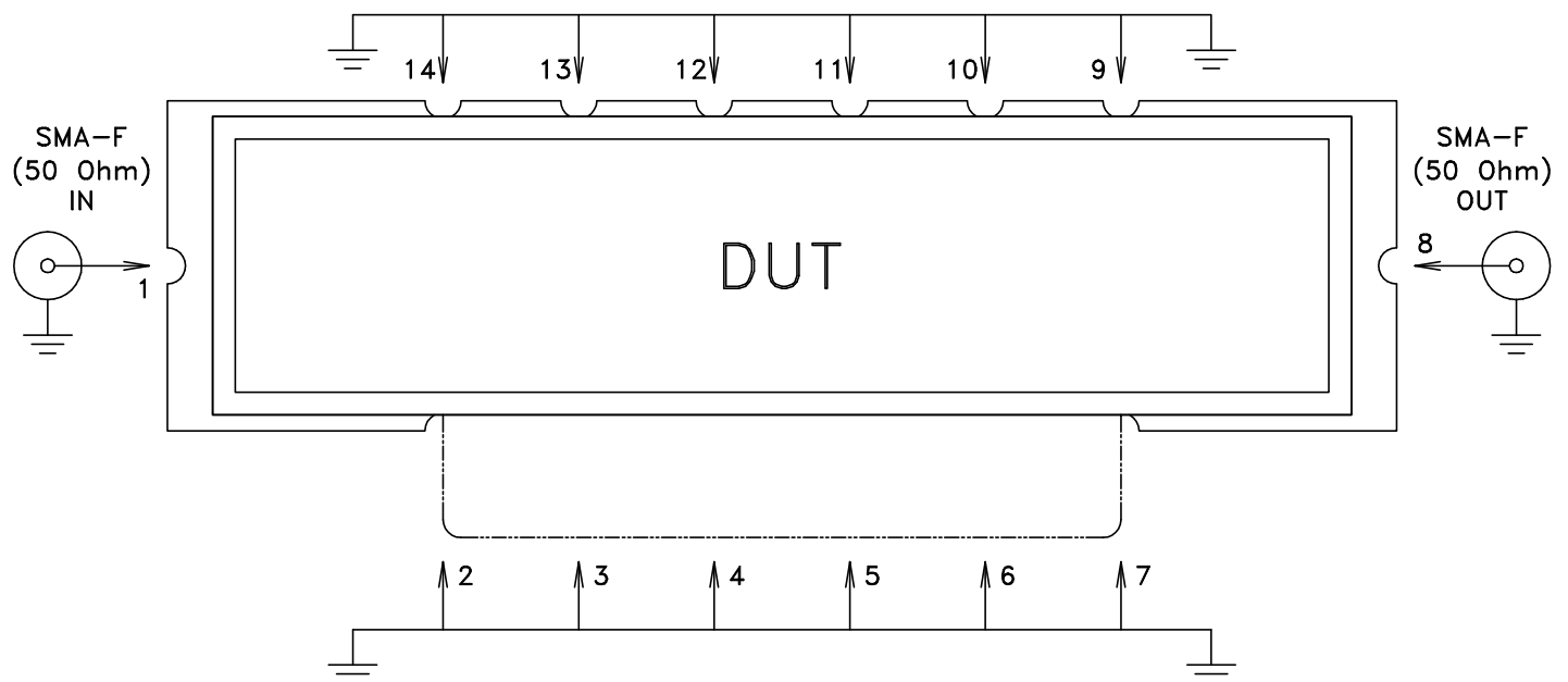
Schematic Diagram
