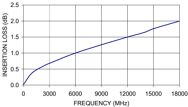
CBL3NMQ-SM+ INSERTION LOSS
