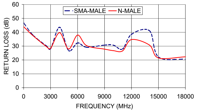
CBL3NMQ-SM+ RETURN LOSS
