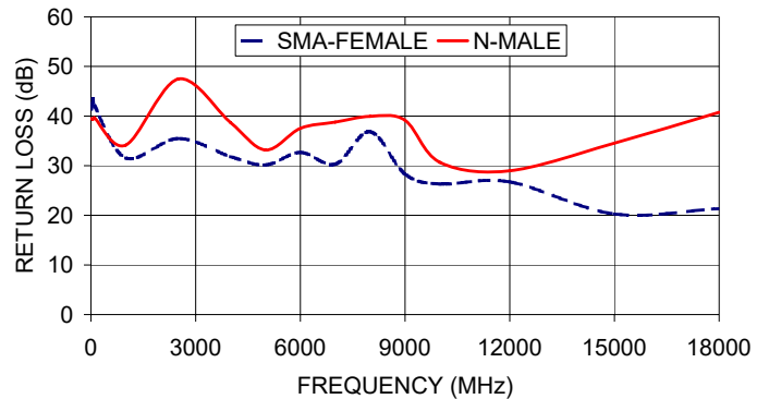
CBL-6FT-SFNM+ RETURN LOSS
