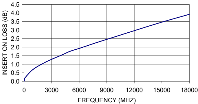
CBL-6FT-SFNM+ INSERTION LOSS
