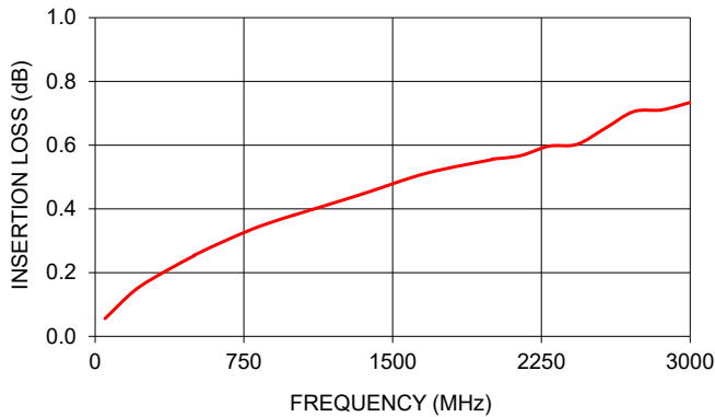
CBL-3FM-75+ INSERTION LOSS
