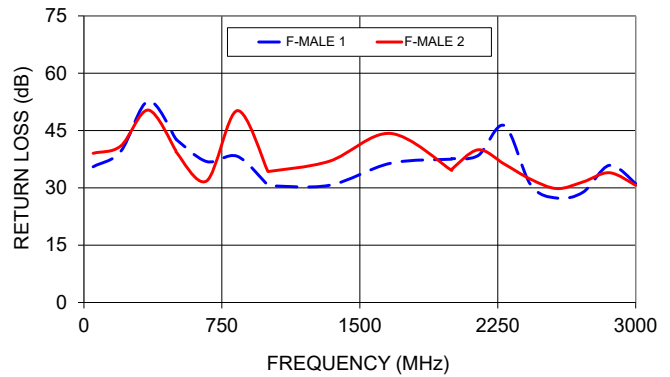
CBL-3FM-75+ RETURN LOSS
