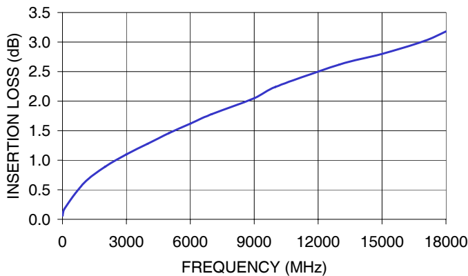
CBL-1.5M-SMNM+ INSERTION LOSS
