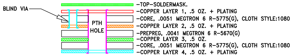
STACK-UP DIAGRAM
