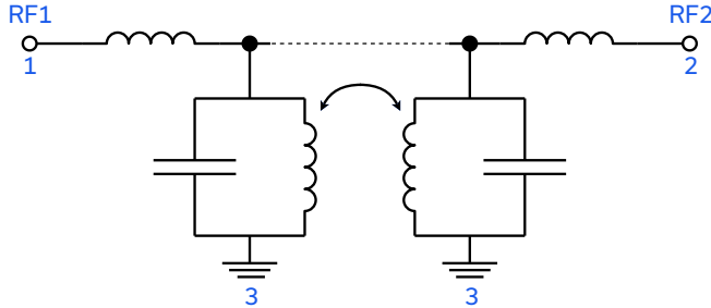
Figure 1. BFHK-7551+ Functional Diagram
