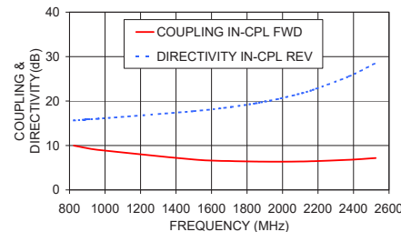
BDCN-7-25+ COUPLING & DIRECTIVITY
