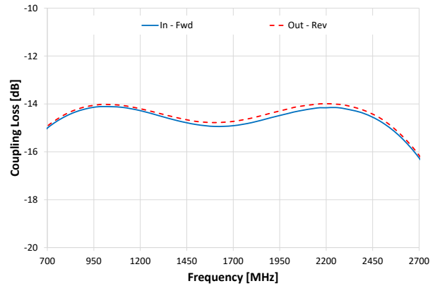
Coupling Loss vs. Frequency
