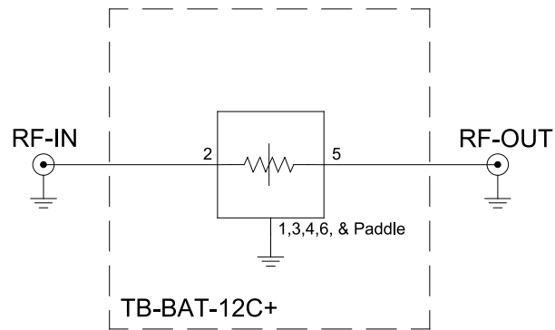
Figure 2. BAT-12+ Characterization and Application Circuit.
