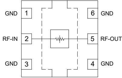
Figure 1. BAT-10+ Functional Diagram
