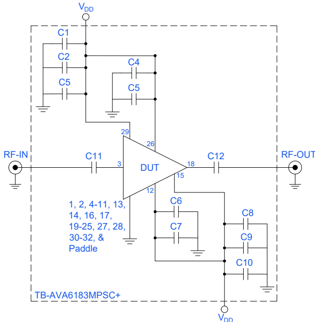
Figure 2. AVA-6183MPS+ Evaluation and Application Circuit
