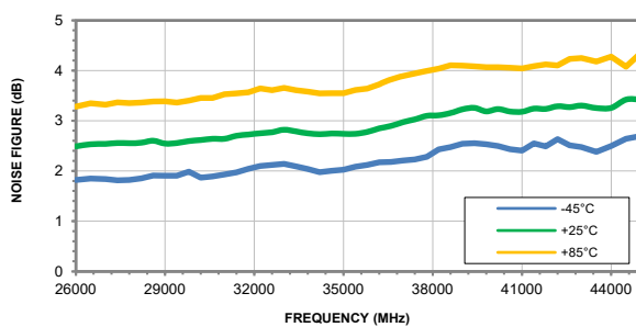
NOISE FIGURE vs. FREQUENCY & TEMPERATURE VDD = +3V
