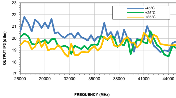
OUTPUT IP3 vs. FREQUENCY & TEMPERATURE @ VDD = +3V
