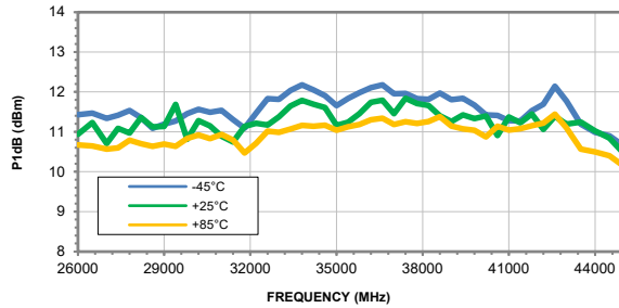
P1dB vs. FREQUENCY & TEMPERATURE VDD = +3V
