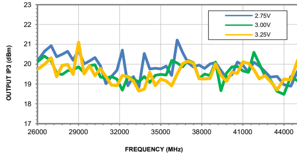
OUTPUT IP3 vs. FREQUENCY & DEVICE VOLTAGE Temperature = +25°C
