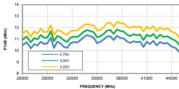
P1dB vs. FREQUENCY & DEVICE VOLTAGE Temperature = +25°C
