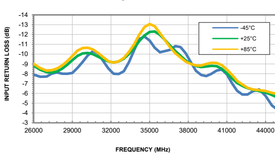
INPUT RETURN LOSS vs. FREQ. & TEMP. @ VDD = +3V
