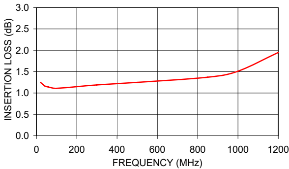
ADT1.5-122+ INSERTION LOSS
