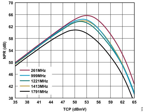
Figure 13. NPR vs. TCP Over Frequency, 0 dB Tilt
