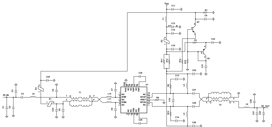
Figure 38. Downstream Application Circuit with Active Biasing Schematic
