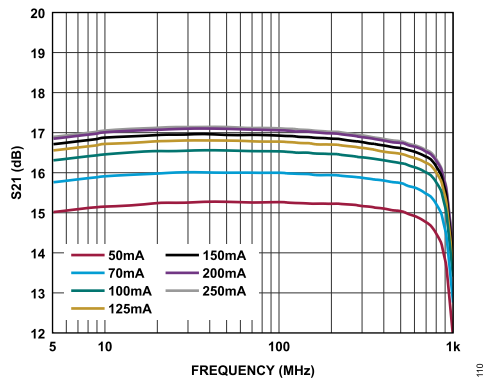
Figure 10. Upstream S21 vs. Frequency Over Bias Current
