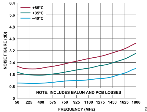
Figure 33. Noise Figure vs. Frequency Over Temperature, V_{DD} = 5.0 V, I_{DD} = 250 mA
