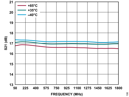
Figure 6. Downstream S21 vs. Frequency Over Temperature
