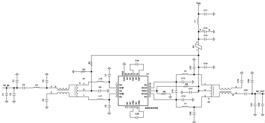
Figure 39. Upstream Application Circuit with Passive Biasing Schematic
