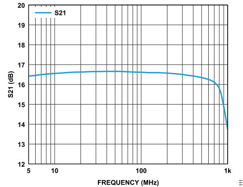
Figure 11. Upstream S21 vs. Frequency
