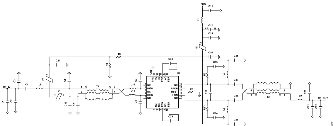
Figure 37. Downstream Application Circuit with Passive Biasing Schematic
