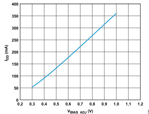
Figure 36. I_{DD} vs. V_{BIAS\_ADJ}
