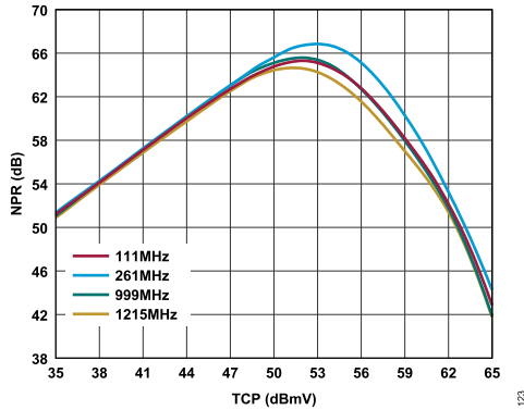
Figure 23. NPR vs. TCP Over Frequency, 0 dB Tilt
