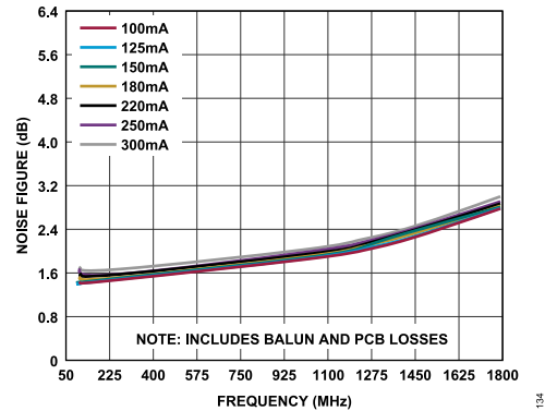
Figure 34. Noise Figure vs. Frequency Over Current, V_{DD} = 5.0 V, T_{PADDLE} = 35^\circ\text{C}
