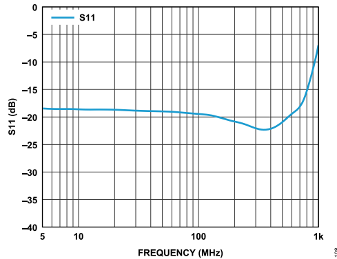
Figure 8. Upstream S11 vs. Frequency
