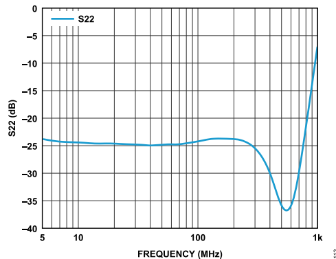
Figure 12. Upstream S22 vs. Frequency
