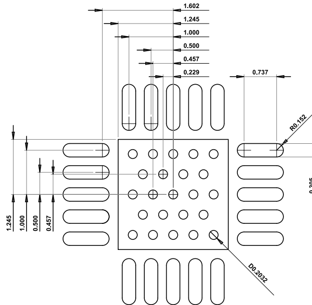
Figure 35. Recommended PCB Layout (Dimensions Shown in Millimeters)
