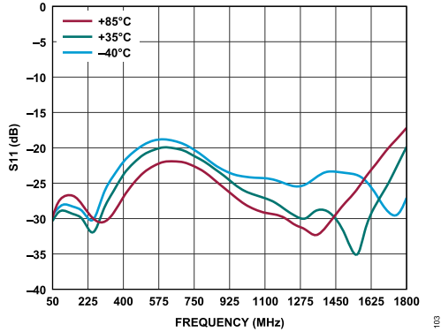
Figure 3. Downstream S11 vs. Frequency Over Temperature
