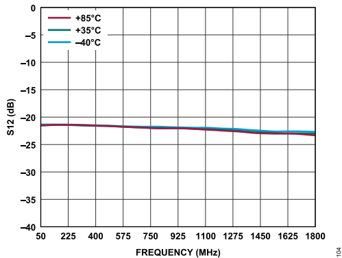
Figure 4. Downstream S12 vs. Frequency Over Temperature
