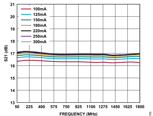
Figure 5. S21 vs. Frequency Over Bias Current
