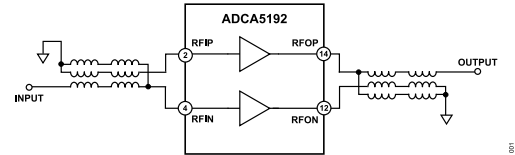
Figure 1. Functional Block Diagram
