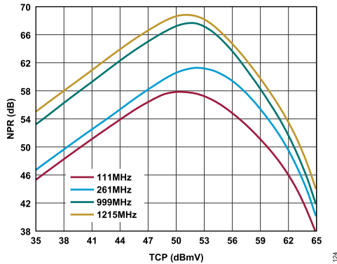
Figure 24. NPR vs. TCP Over Frequency, 10 dB Tilt
