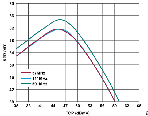
Figure 29. NPR vs. TCP Over Frequency, 3 dB Tilt
