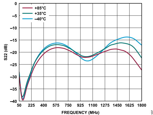
Figure 7. Downstream S22 vs. Frequency Over Temperature
