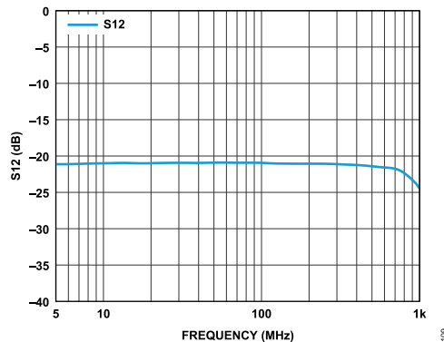
Figure 9. Upstream S12 vs. Frequency
