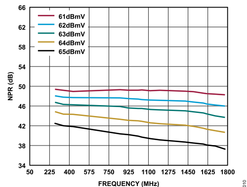
Figure 10. NPR vs. Frequency Over TCP, 10 dB Tilt, No Offset at 1026 MHz, V_{DD} = 5.0\text{ V} , I_{DD} = 250\text{ mA}
