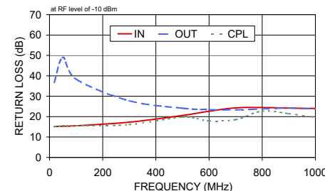
ADC-6-10-75+ RETURN LOSS
