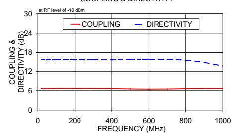
ADC-6-10-75+ COUPLING & DIRECTIVITY
