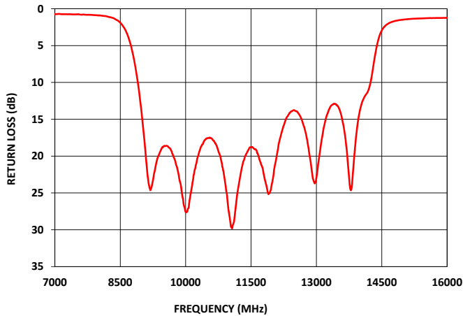
ABF-11R5G+ RETURN LOSS
