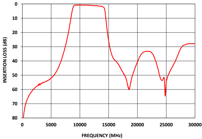
ABF-11R5G+ INSERTION LOSS
