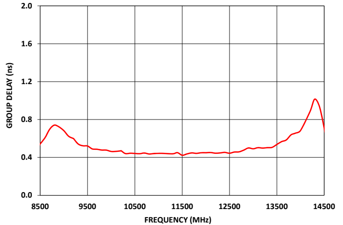
ABF-11R5G+ GROUP DELAY
