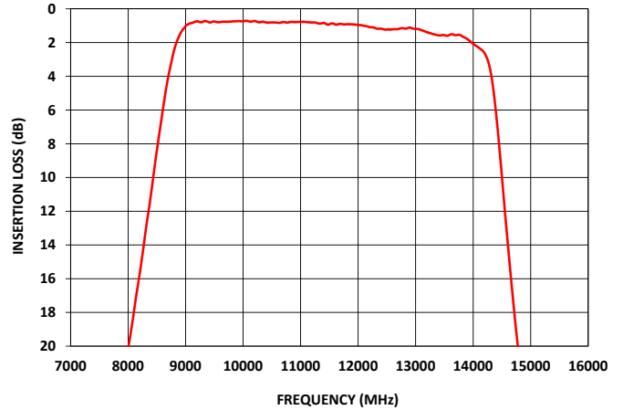
ABF-11R5G+ INSERTION LOSS (Zoomed)
