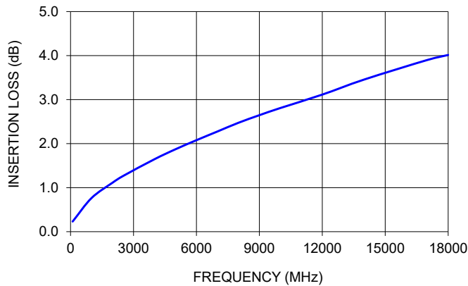
141-72SM+ INSERTION LOSS
