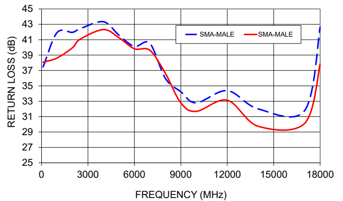
141-72SM+ RETURN LOSS
