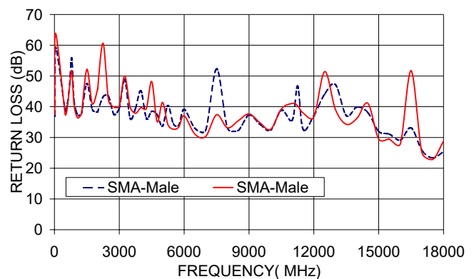
141-6SM+ RETURN LOSS
