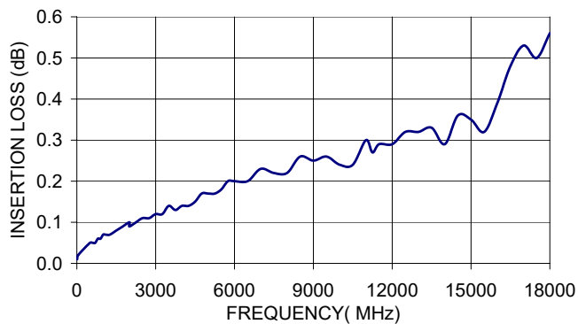
141-6SM+ INSERTION LOSS
